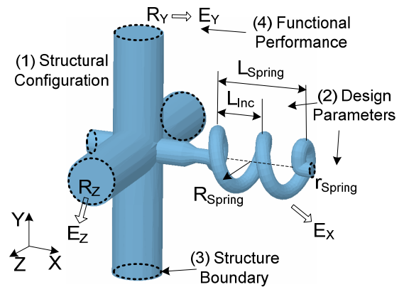
Fig. 4: An example of a performance-tailored mesostructure that is used to generate the CAD model as shown in Figure 1.
