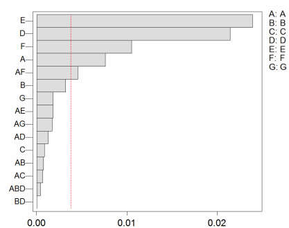
Fig. 6: Pareto chart of the parameter effect related to the central displacement.
