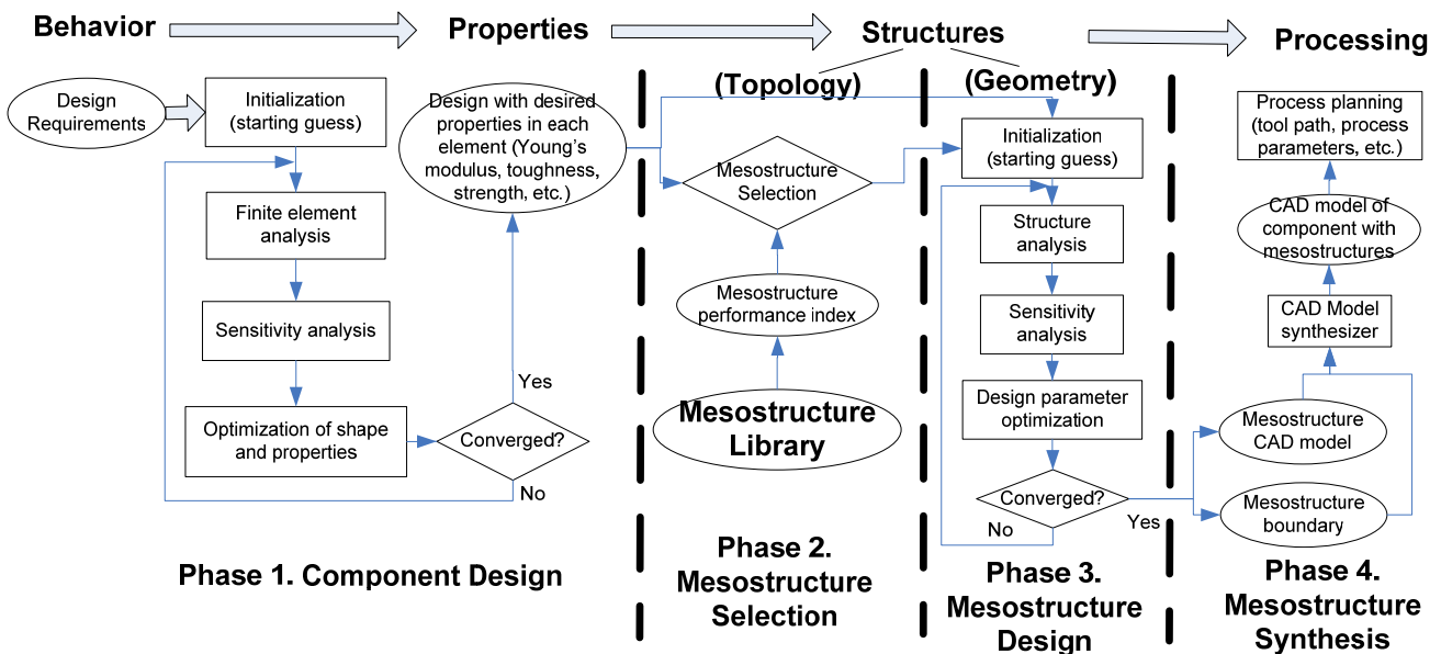
Fig. 12: A design framework based on the performance-tailored mesostructures.
