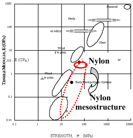
Fig. 9: An illustrative example of applying Ashby chart for the mesostructure selection.
