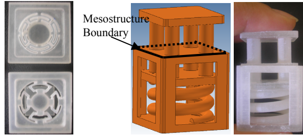
Fig. 8: (left) A photo of the built mesostructure with two sets of parameter values; (right) a mesostructure with spring design that can achieve a bigger central displacement than the mesostructure as shown in Figure 5.
