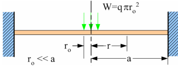
Fig. 7: A clamped circular plate under distributed body force [18].
