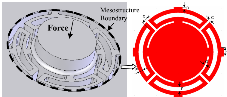
Fig. 5: A mesostructure and its design parameters based on a diaphragm flexure design [17].
