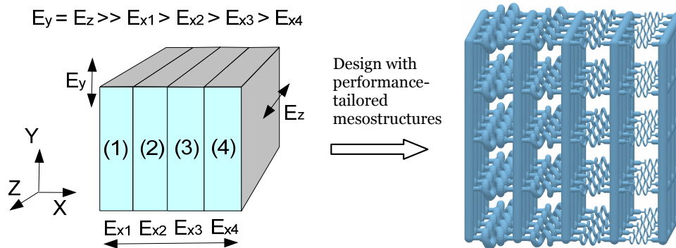
Fig. 1: An illustration of the performance-tailored mesostructures to achieve heterogeneous material properties. Suppose the designer specifies a simple cube design (left), in which, the material's Young's modulus in Y and Z axes is much bigger than that in X axis; further, the material's Young's modulus needs to decrease along X axis. Based on the desired material properties, a CAD model generated by our approach for the cube design is shown in the figure (right).
