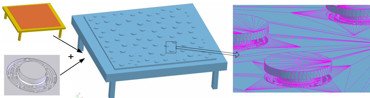
Fig. 14: A chair example with performance-tailored mesostructures.
