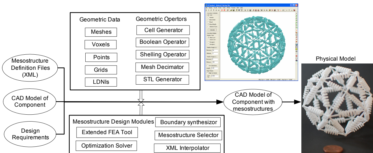
Fig. 13: A CAD system for component design based on performance-tailored mesostructure.
