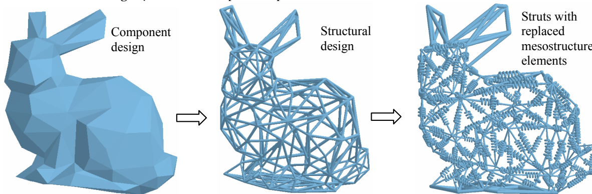
Fig. 15: A bunny example with performance-tailored mesostructures.
