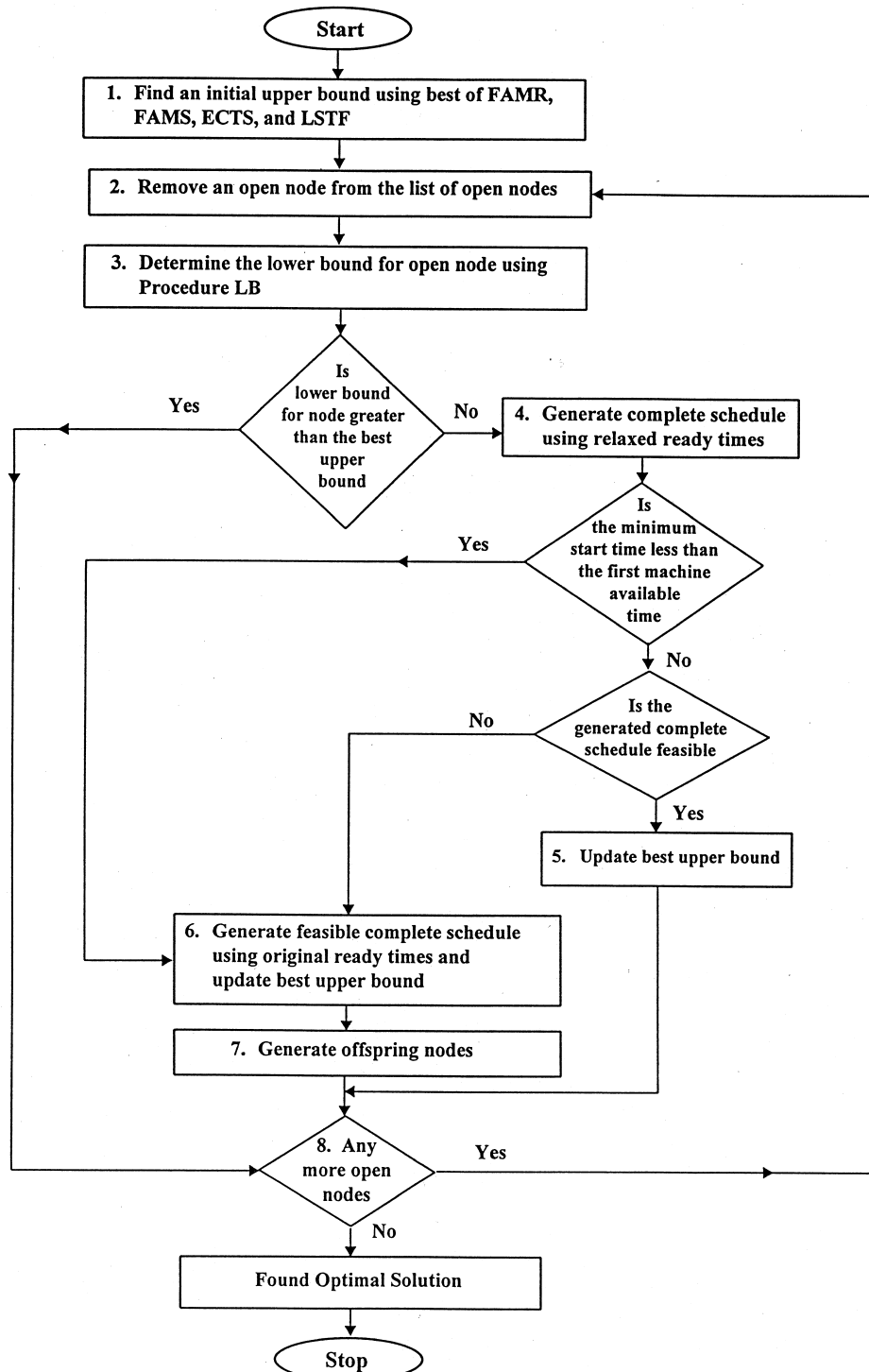
Fig. 1. Overview of branch-and-bound procedure.
