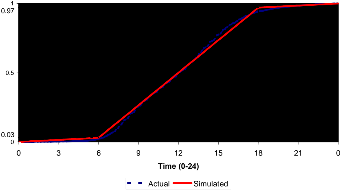
Figure 8 ó Actual and simulated cumulative distribution of requested pick-up time
