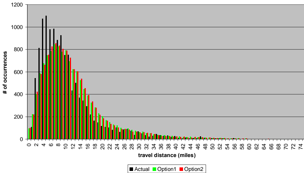
Figure 9 ó Comparison between actual and simulated travel distance distributions
