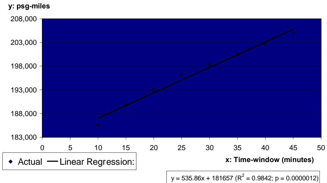
Figure 13 ó Linear regression: passenger-miles
