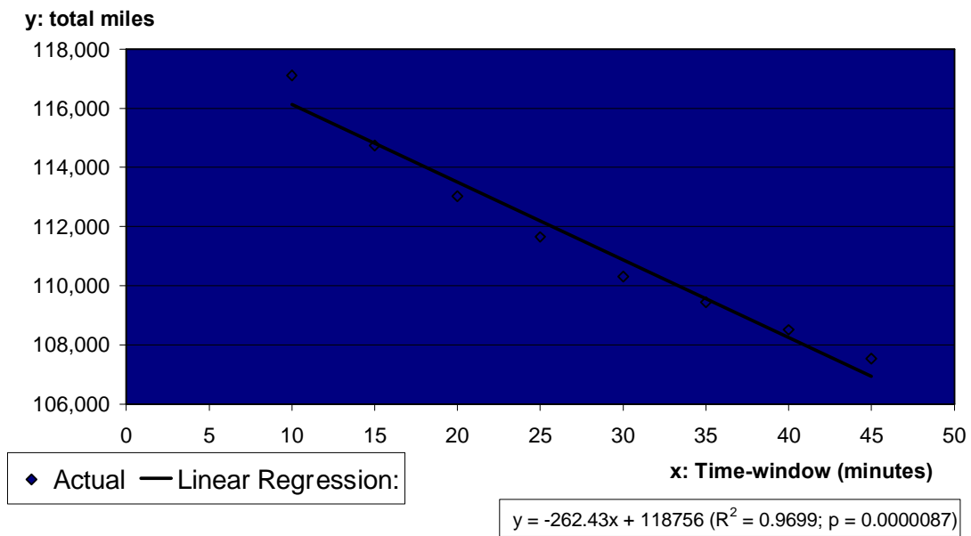
Figure 11 ó Linear regression: total miles
