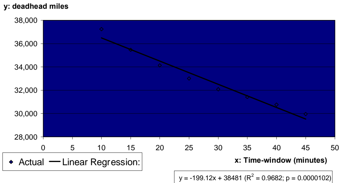
Figure 12 ó Linear regression: deadhead miles
