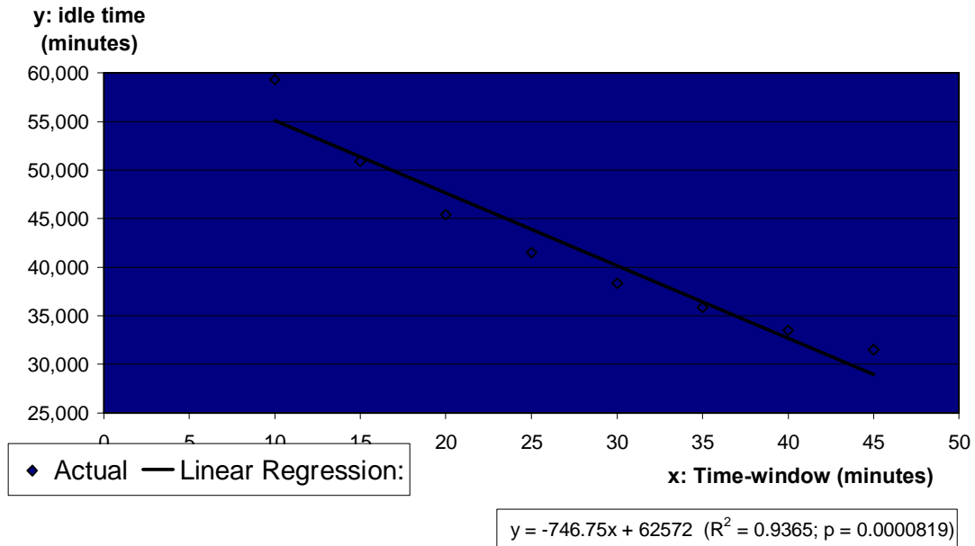
Figure 14 ó Linear regression: idle time (minutes)
