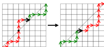
Figure 3. The green and red portions are being exchanged.
