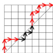
Figure 2. A path with exceedance 5.
