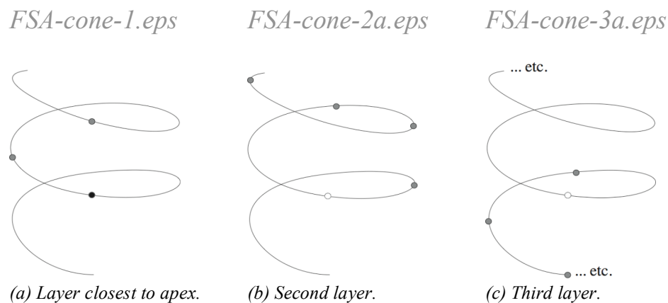
Figure 13. From the Spiral Array to Krumhansl's Pitch Class Cone.
