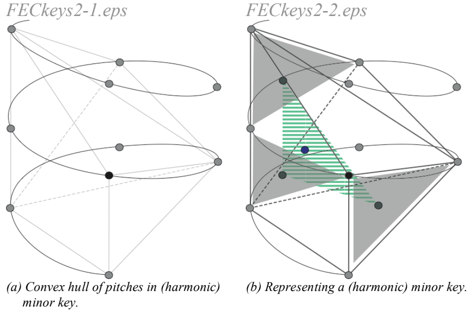
Figure 7. Minor key span and representation in the Spiral Array.
