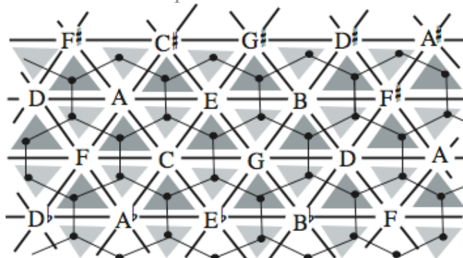
Figure 2. Triads form the dual graph of the Harmonic Network.
