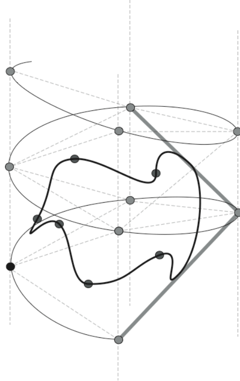
Figure 17. Lerdahl's Chordal Space mapped to the Spiral Array.
