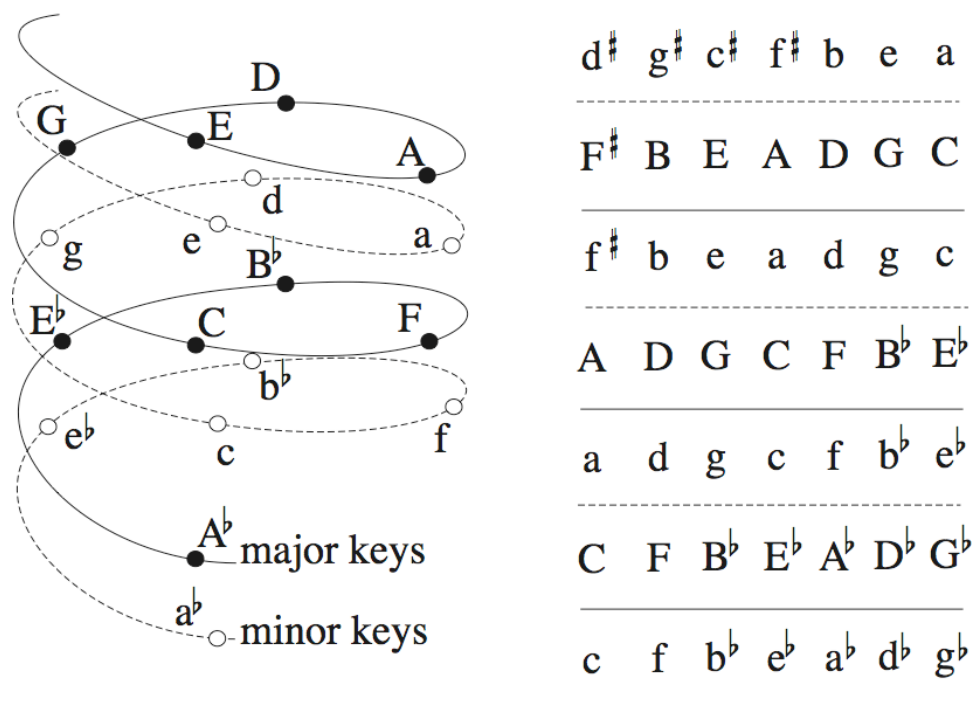
Figure 18. Key Representations in the Spiral Array and Lerdahl's Regional Space.
