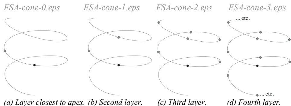
Figure 14. From the Spiral Array to Lerdahl's Pitch Class Cone.
