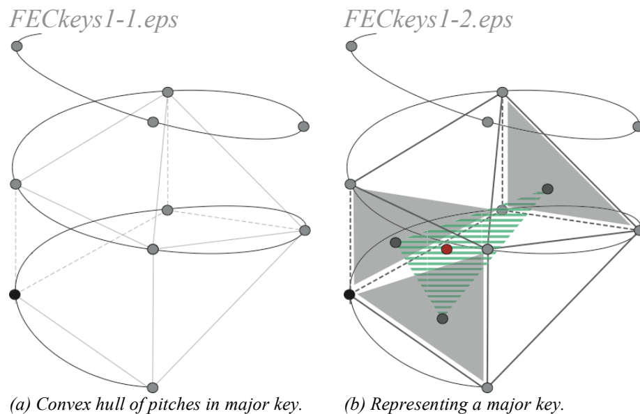
Figure 6. Major key span and representation in the Spiral Array.
