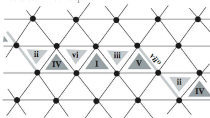
Figure 16. Lerdahl's Chord Space mapped to the Harmonic Network.
