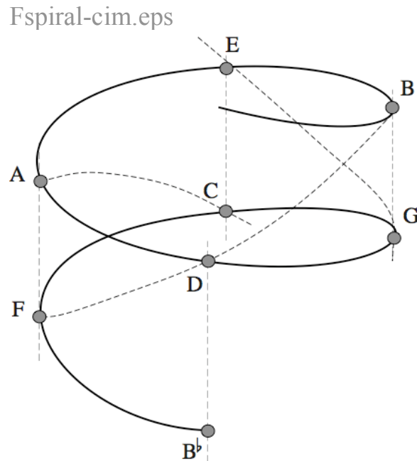
Figure 4. Spiral representation of the Harmonic Network.
