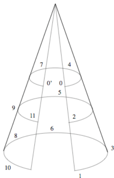
(a) Krumhansl's pitch cone (inverted).
