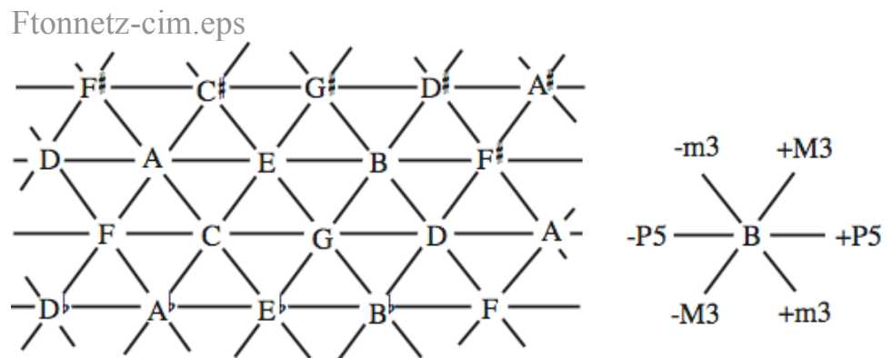
Figure 1. The Harmonic Network, also known as the Tonnetz .
