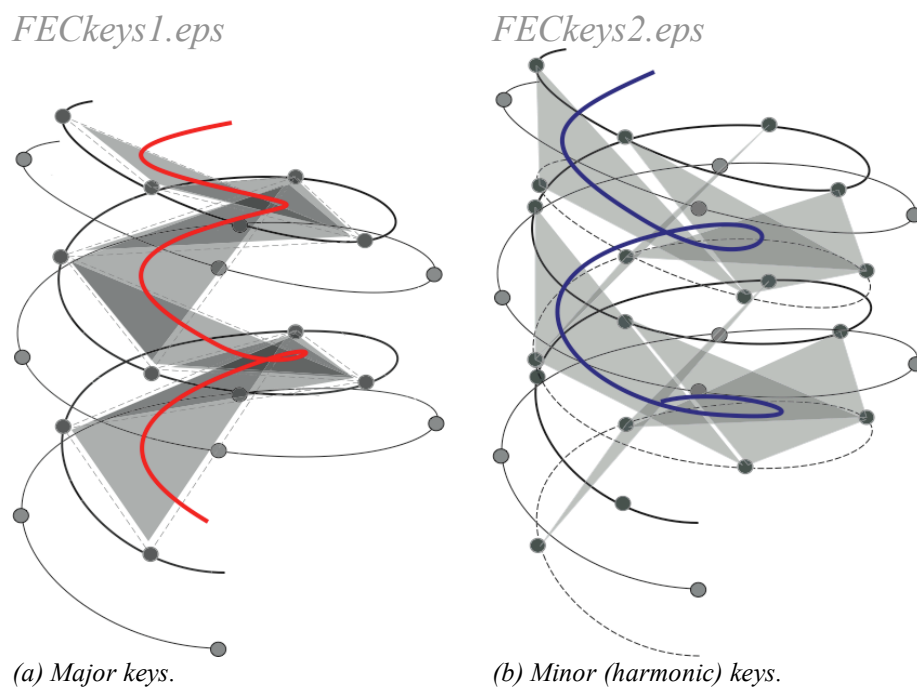
Figure 8. Key Representations in the Spiral Array.
